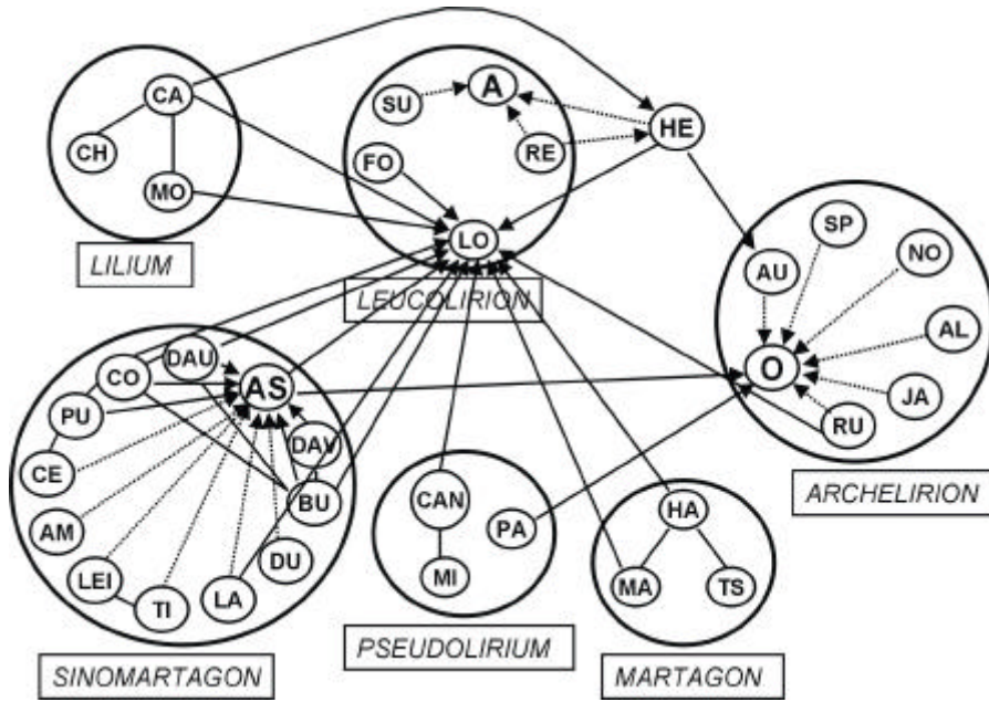
Figure 19-1. A crossing polygon of the genus Lilium including all successful crosses of species between different sections of the genus Lilium developed at Plant Research International, The Netherlands. In this figure, the connection between the Asiatic, Aurelian, and Oriental hybrid groups (large ellipses) are shown by dotted lines. In successful crosses between species (small circles) of different sections (large circles) the arrows point towards the female parent. Abbreviations: A: Aurelian hybrids; AL: L. alexandrae ; AM: L. amabile ; AS: Asiatic hybrids; AU: L. auratum ; BU: L. bulbiferum ; CA: L. candidum ; CAN: L. canadense ; CE: L. cernuum ; CH: L. chalcedonicum ; CO: L. concolor ; DAU: L. dauricum ; DAV: L. davidii ; DU: L. duchartrei ; FO: L. formosanum ; HA: L. hansonii ; HE: L. henryi ; JA: L. japonicum ; LA: L. lankongense ; LEI: L. leichtlinii ; LO: L. longiflorum ; MA: L. martagon ; MI: L. michiganense ; MO: L. monadelphum ; NO: L. nobilissimum ; O: Oriental hybrids; PA: L. pardalinum ; PU: L. pumilum ; RE: L. regale ; RU: L. rubellum ; SP: L. speciosum ; SU: L. sulphureum ; TI: L. tigrinum ; TS: L. tsingtauense .
